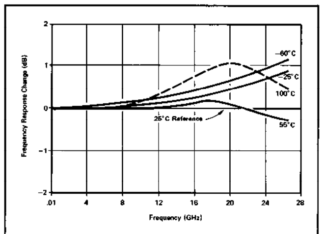
Figure 8. Typical Frequency Response Variation with Temperature.
