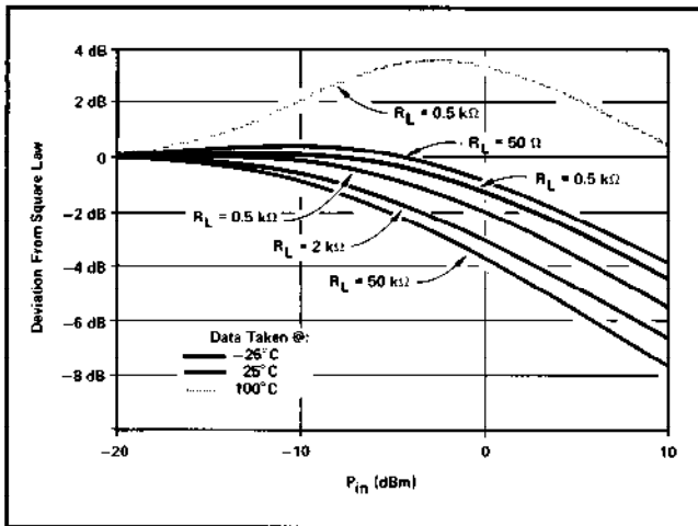
Figure 4. Typical Square Law Deviation.
