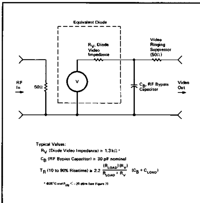
Figure 1. Equivalent Circuit for 33330B/C Detectors with Typical Parameter Values.
