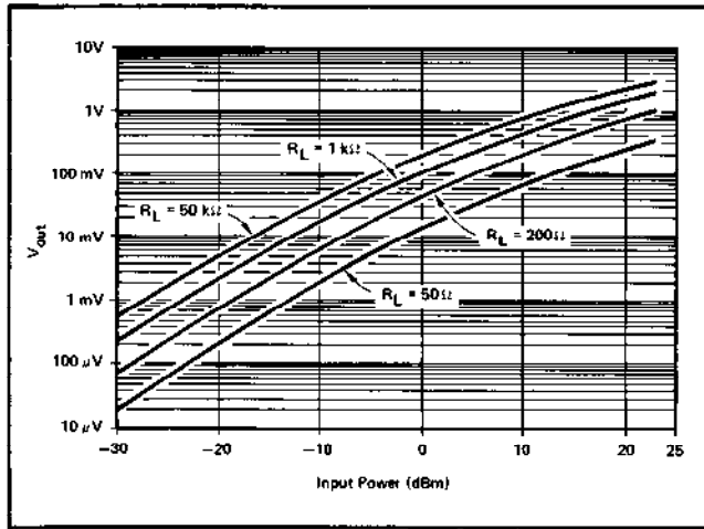
Figure 3. Typical Transfer Characteristics. ( T_a = 25^\circ\text{C} )
