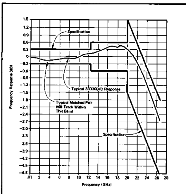
Figure 2. Typical Frequency Response of 33330B/C Detectors.
