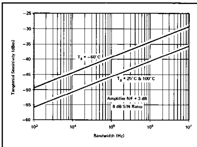
Figure 5. Typical Tangential Sensitivity.
