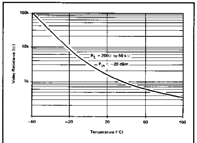
Figure 7. Typical Video Impedance Variation with Temperature.
