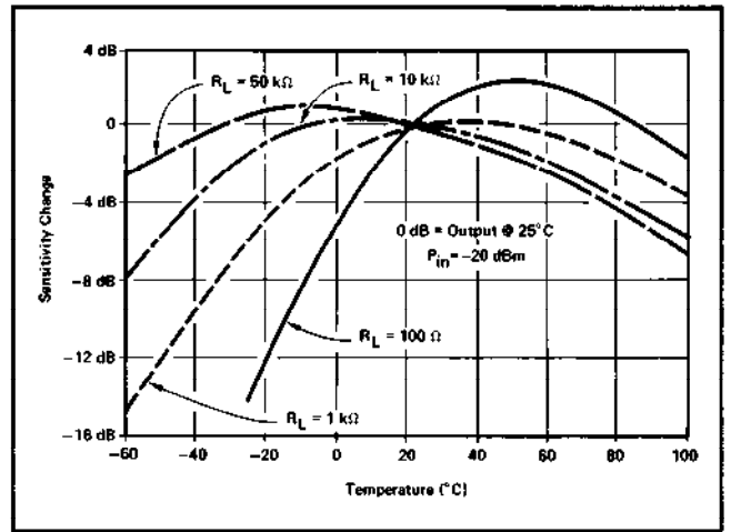
Figure 6. Typical Output Response with Temperature. ( P_{in} < -20\text{ dBm} )
